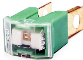
MALE FUSE
